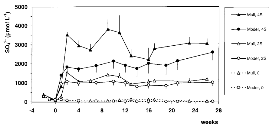
Figure 2. Sulphate ( \text{SO}_4^{2-} ) concentrations in the pore water of Rhizomull (Mull) and Hydromoder (Moder) soils (see Figure 1) during waterlogging treatment with 0, 2 or 4 \text{mmol L}^{-1} \text{SO}_4^{2-} (indicated 0, 2S, 4S). Means are given, with their standard error ( n = 5 and 6 for Mull and Moder, respectively).
